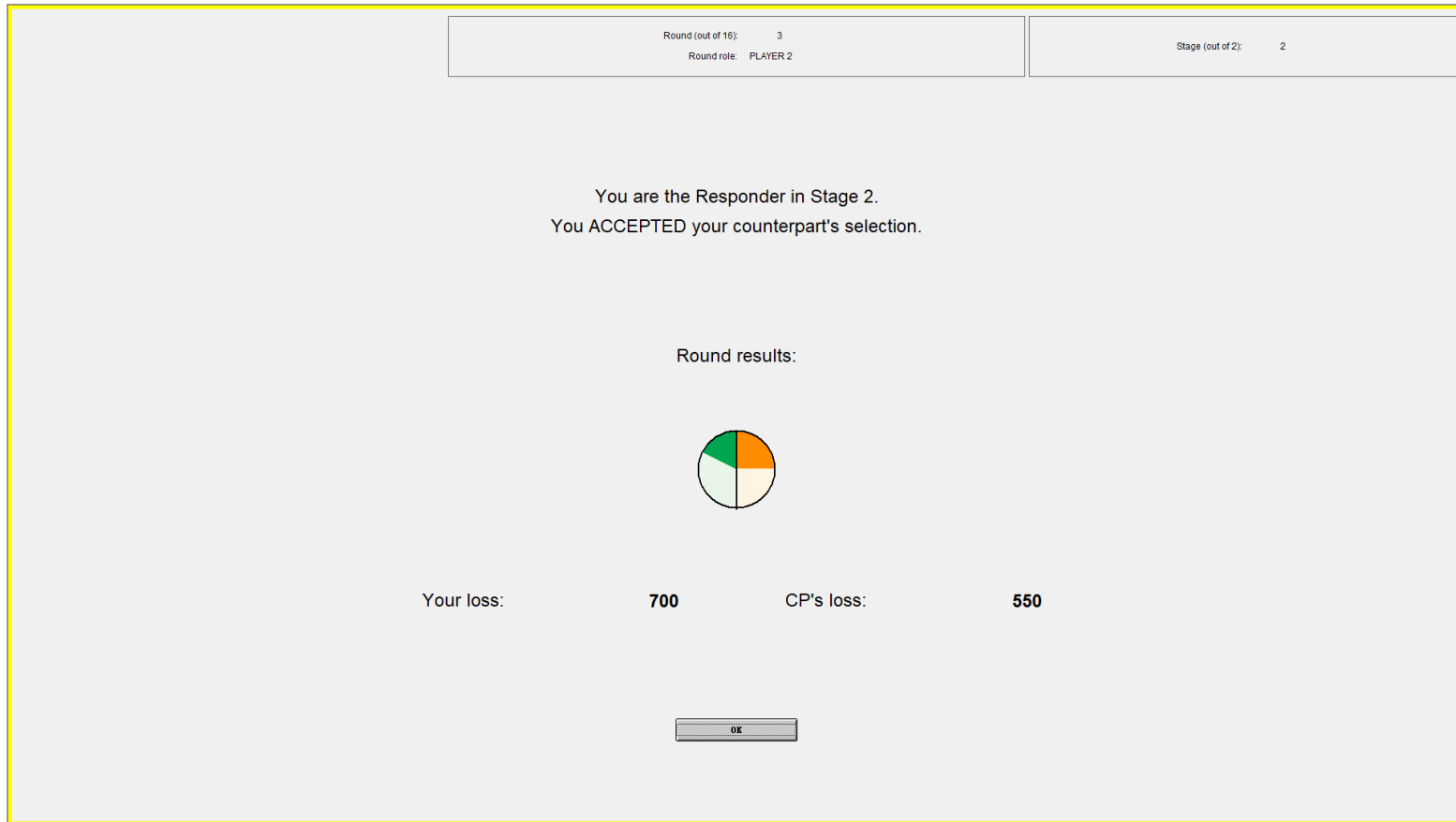
Figure 7: Round Conclusion
